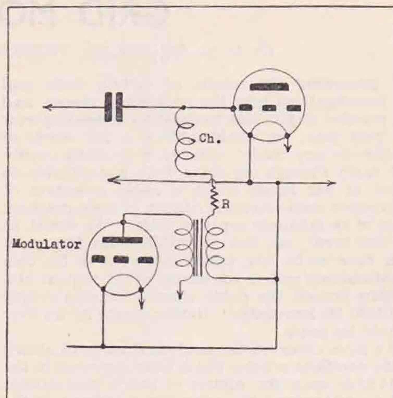
Fig. 4. Modulator Valve working into an incorrect load.
