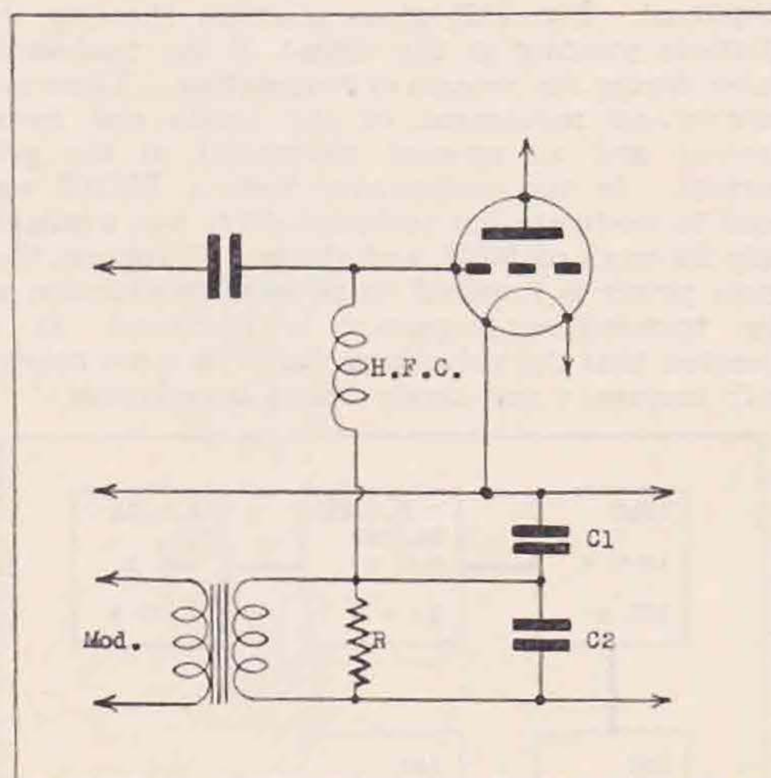
Fig. 14. Application of true grid bias modulation.
