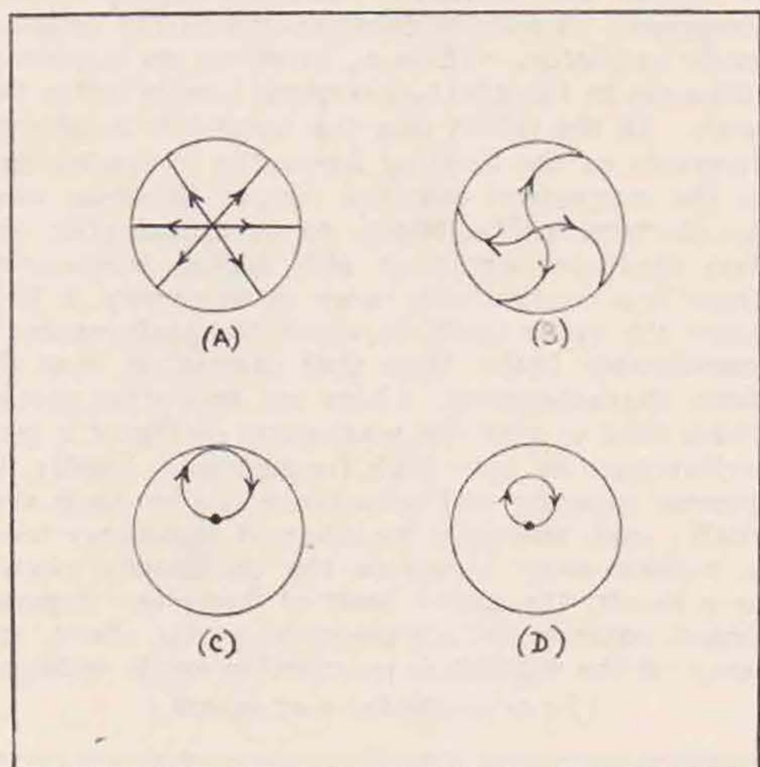
Fig. 3.—Electron paths in a cylindrical diode.
