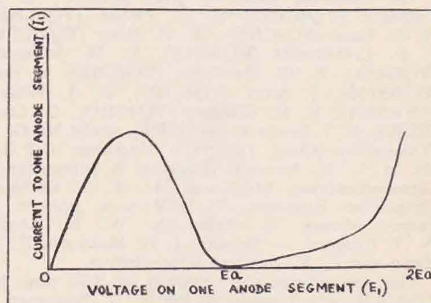
Fig. 6.—Dynatron characteristic of split anode magnetron valve.
