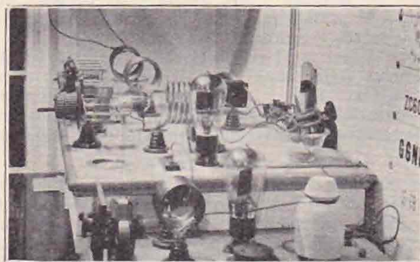
Fig. 5. A general view of the transmitting gear in use at G6LI.
