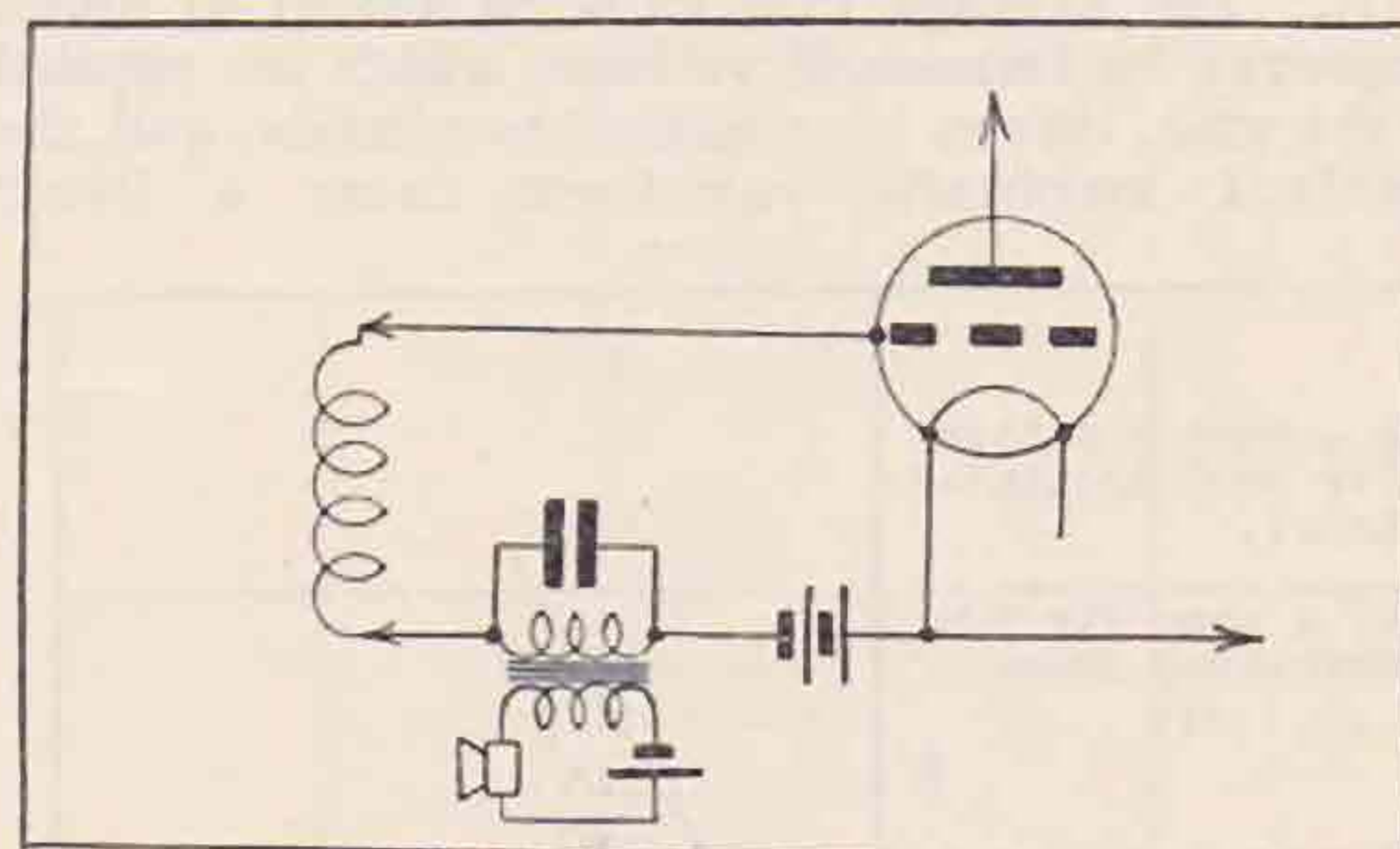
Fig. 1. A simple grid control circuit.
