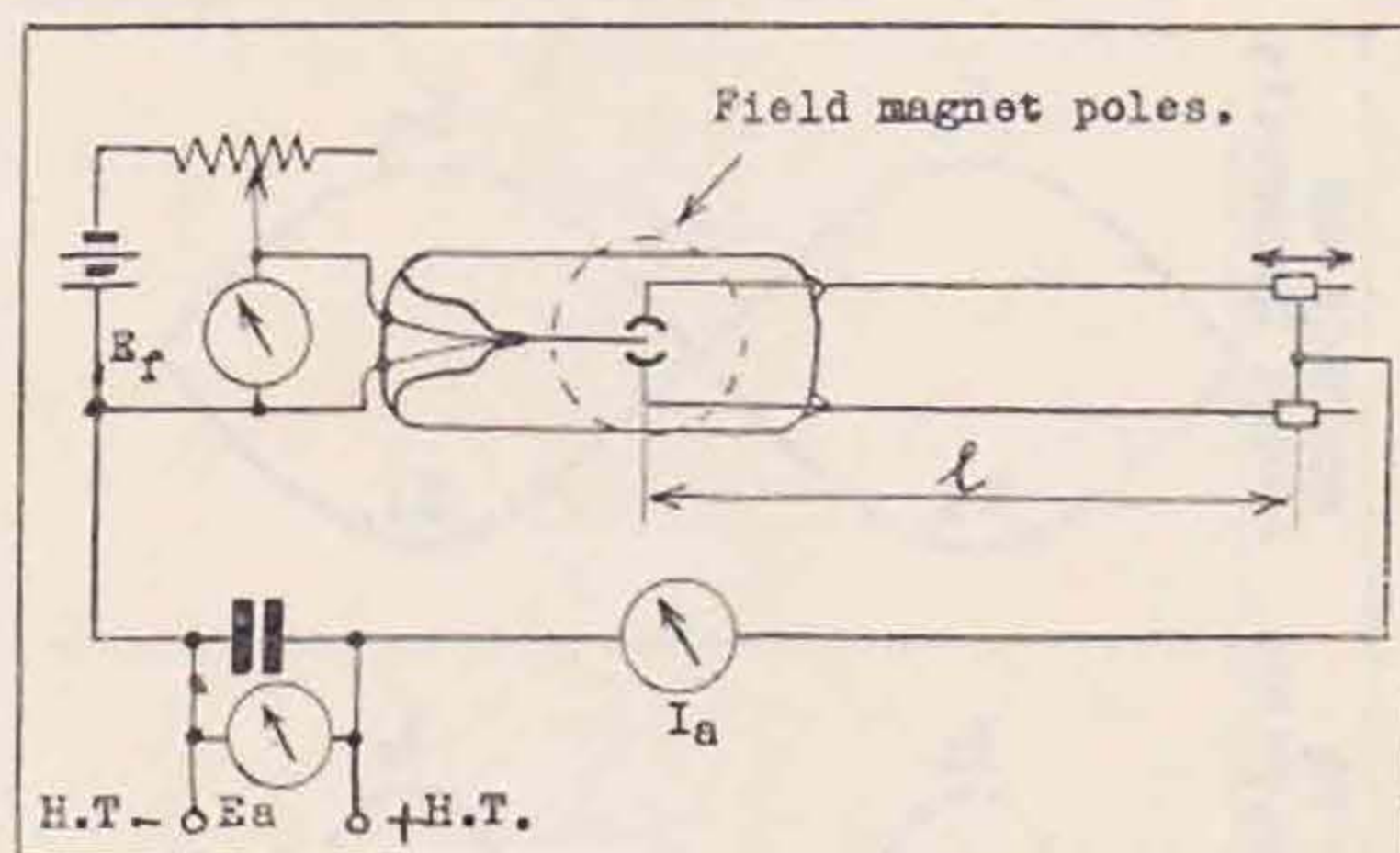
Fig. 5.—Magnetron oscillator circuit for very high frequencies.
